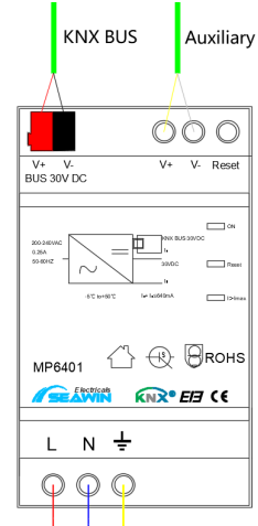
wiring diagram
